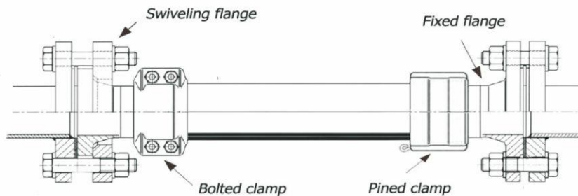
Swivel Flange+clamps
