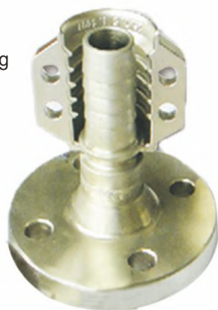
Flange connection
